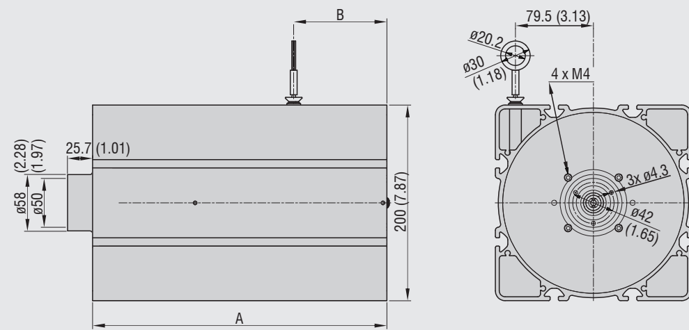
WDS-P200-M series, dimensions in mm (inches)
