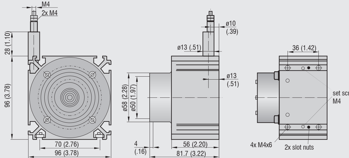
WDS-P96-M series, dimensions in mm (inches)
