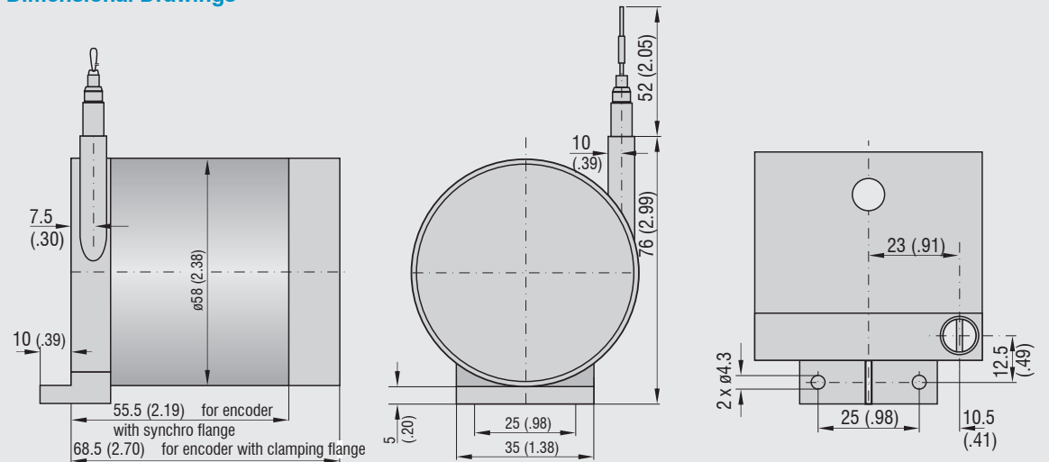
WDS-Z60-M series, dimensions in mm (inches)
